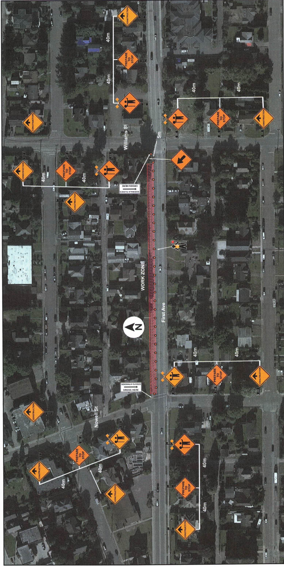
Figure 7.5: Work on Shoulder - Short and Long Duration TCP on site to assist with vehicles, pedestrians, bicyclists and all others
